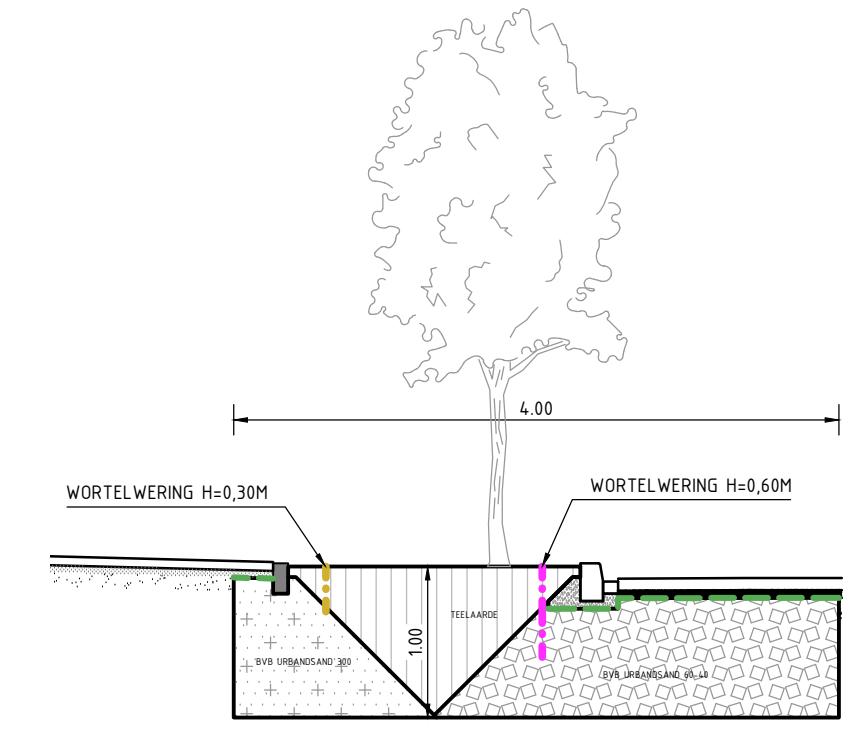
PRINCIPE DETAIL: PLANTVAK LANGS LANGSPARKEREN (1) SCHAAL 150
