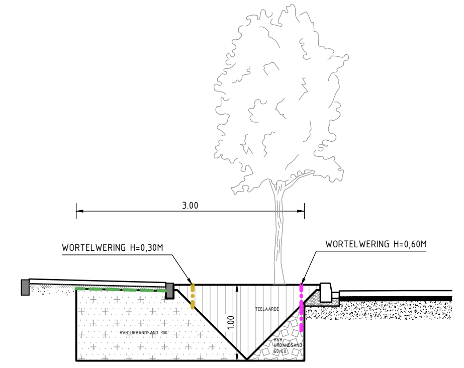
PRINCIPE DETAIL: PLANTVAK LANGS LANGSPARKEREN (2) SCHAAL 150
